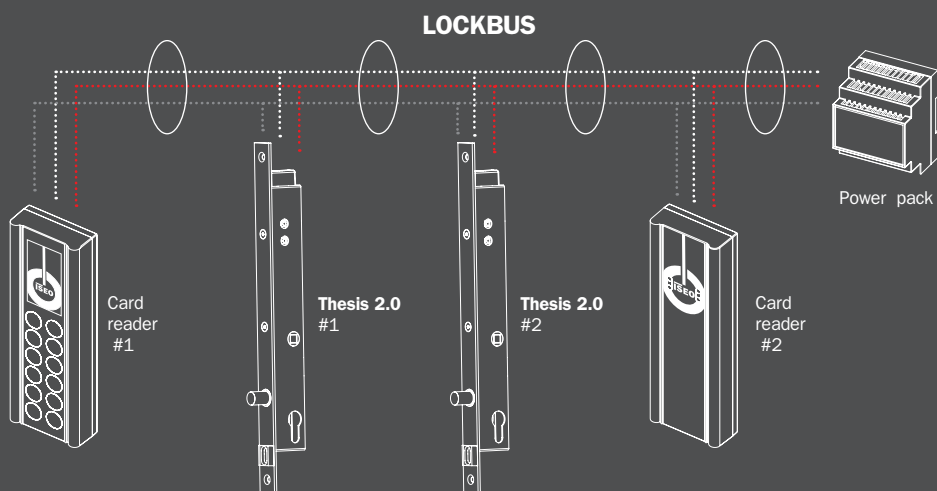
Example of installation of two doors with interlock function
